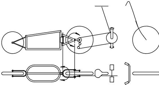
7.2: ONE-WHEEL TRAILER & ATTACHMENT TO BIKE
