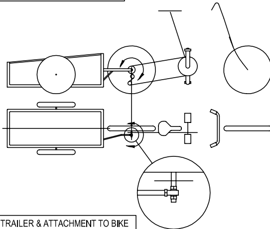
7.2: ONE-WHEEL TRAILER & ATTACHMENT TO BIKE
